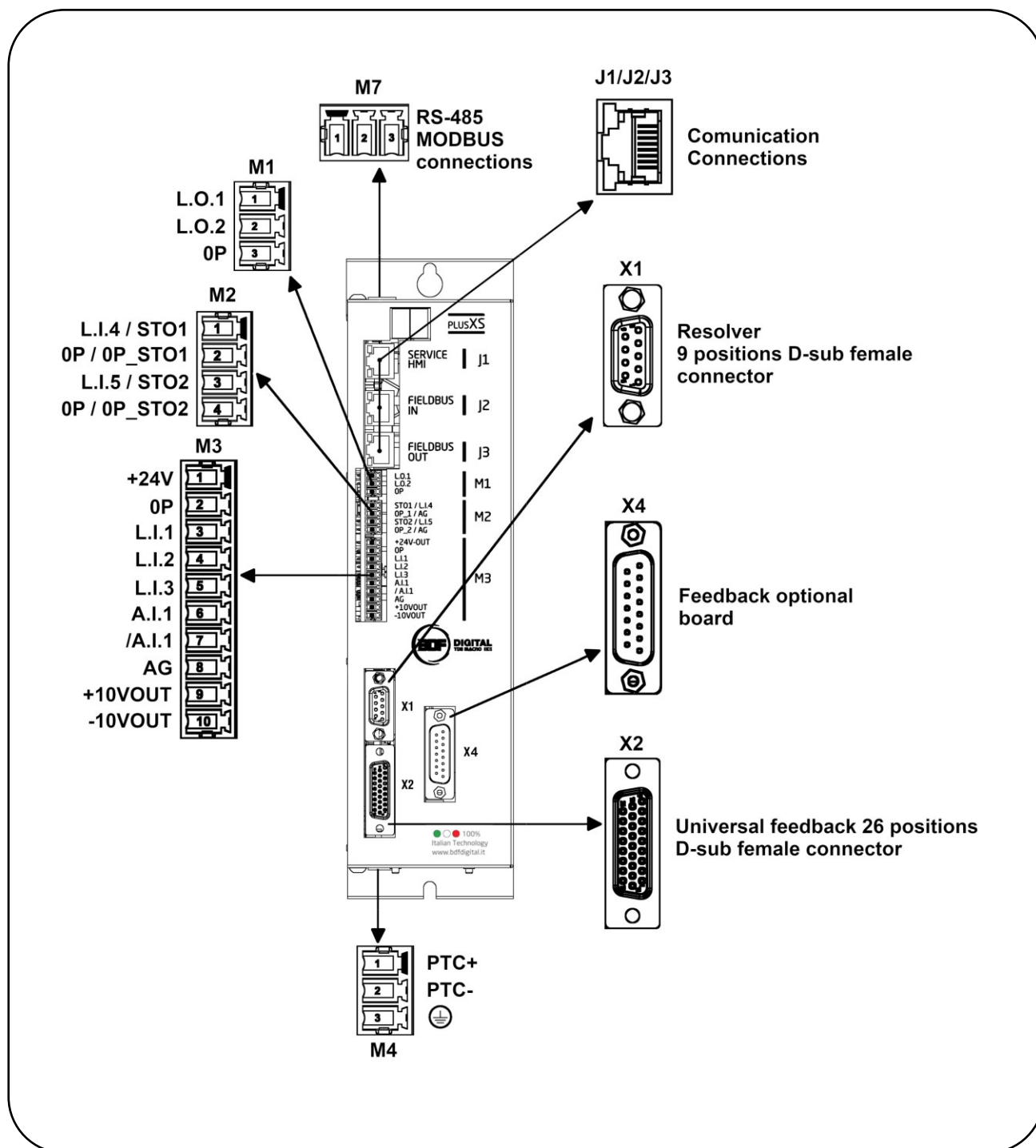
FIG. 24- Collegamenti logici / Logic connections
